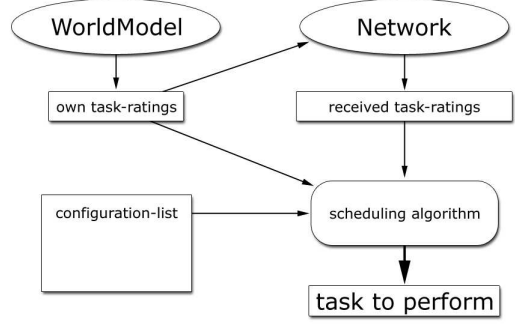
Fig. 2. Schematic view of the scheduling mechanism.
